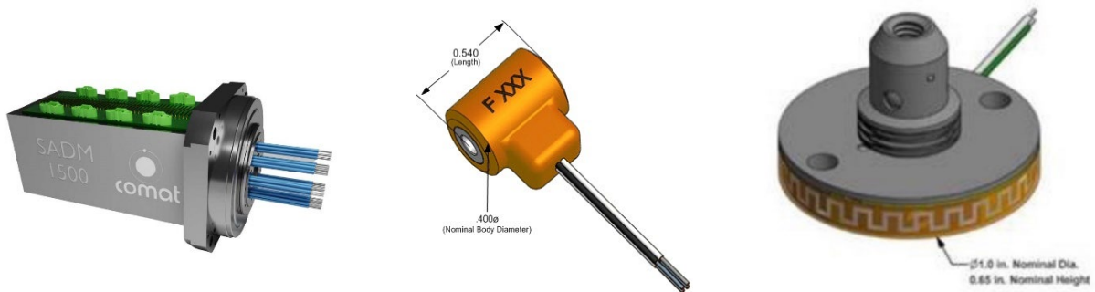
Figure 6.4: (top left) SADM 1500. Credit: Comat. (right) TiNi Aerospace Frangibolt Actuator and (right) ML50 microlatch. Credit: Ensign-Bickford Aerospace & Defense.
