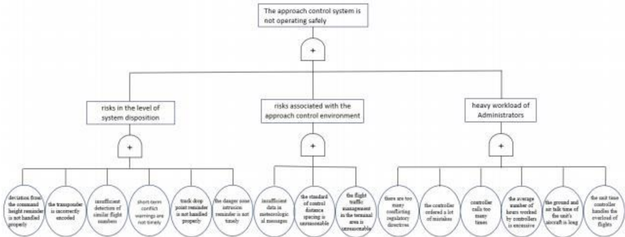
Figure.1. Accident tree of influencing factors for the operation safety
