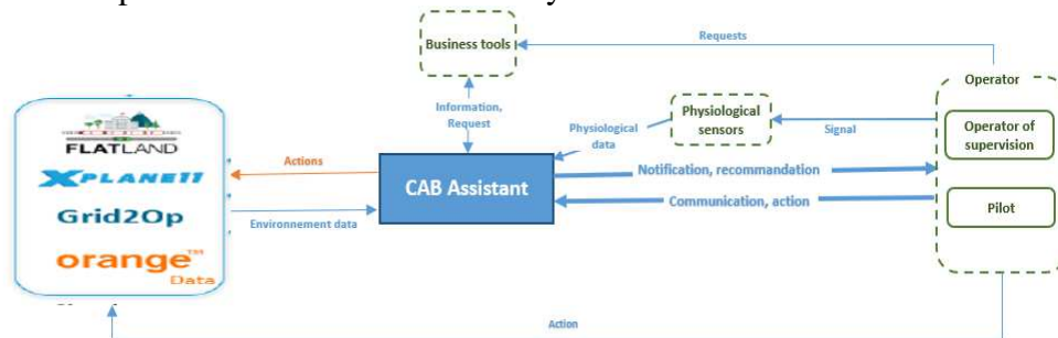
Figure 2. Environment diagram of the CAB assistant
