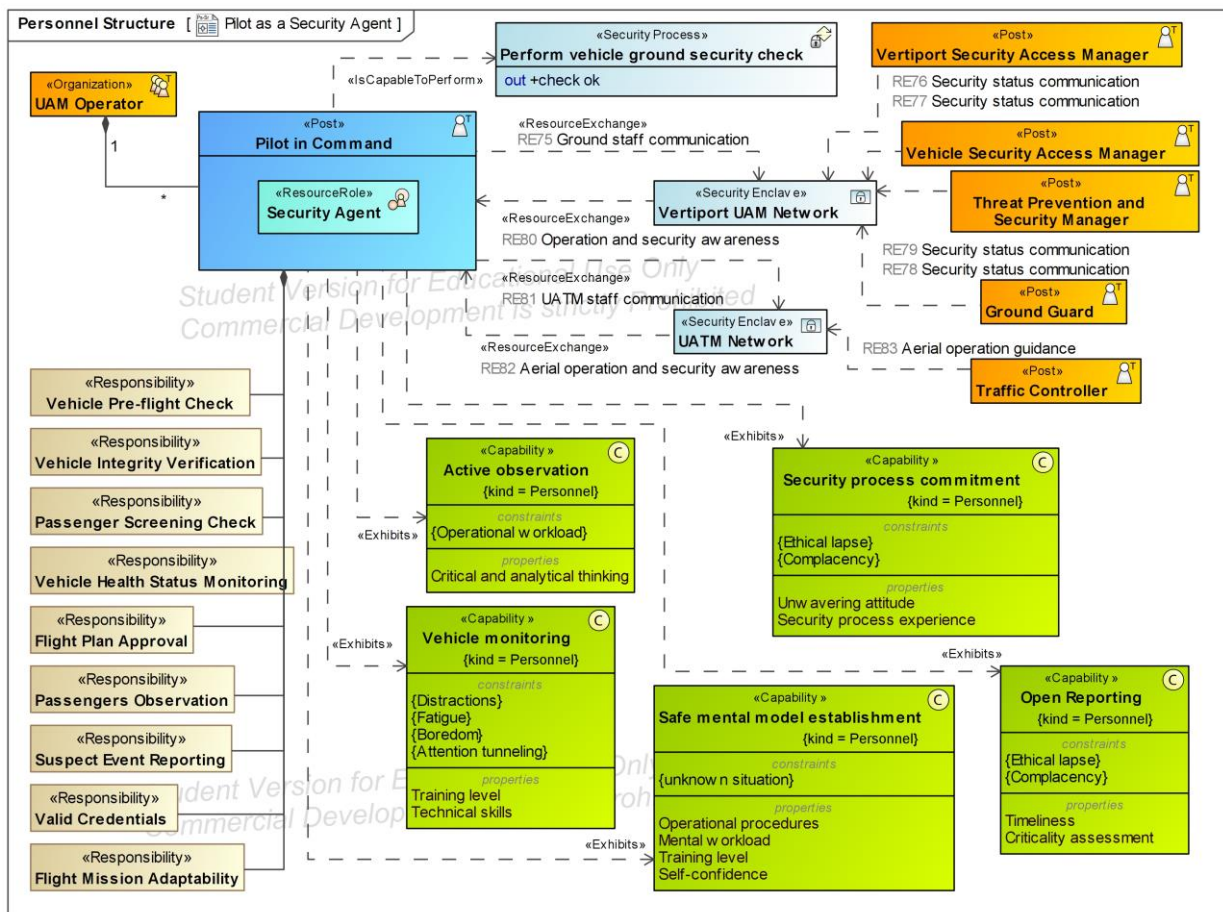
Figure 4. Pilot as a Security Agent
