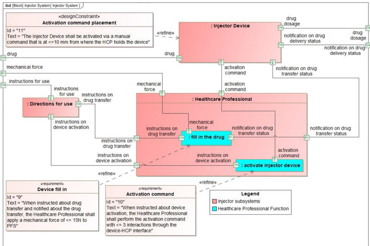
Figure 4. Injector System decomposition
