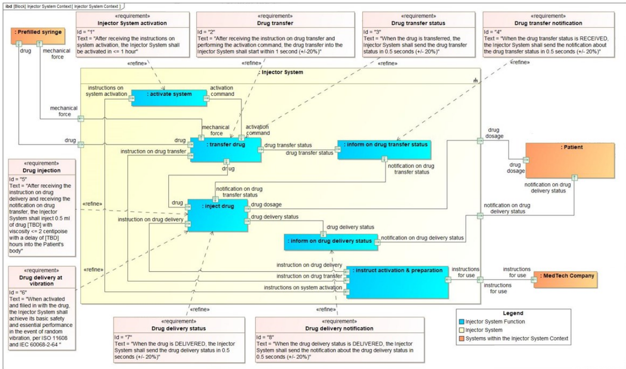
Figure 3. The Injector System Context breakdown decomposition (HCP is inside the SoI)
