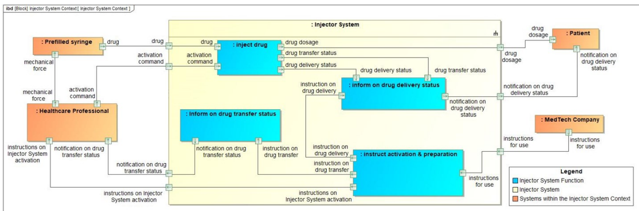
Figure 5. The Injector System Context breakdown decomposition (HCP is outside the SoI)
