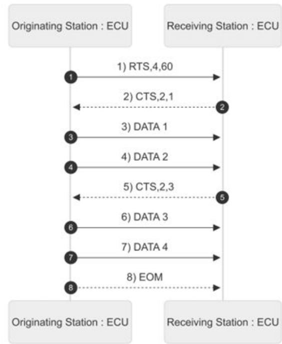
Figure 1. J1587 Connection Mode Data Transfer
