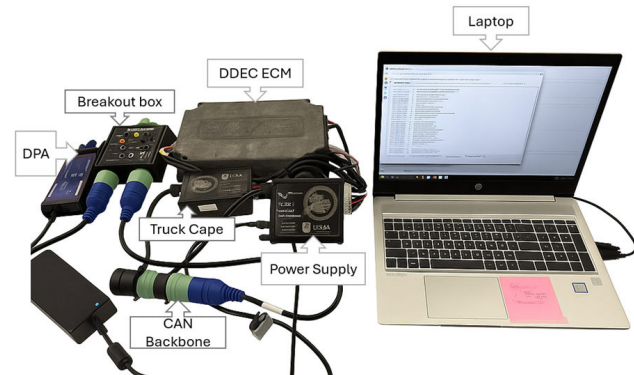
Figure 2. Hardware Setup for J1587/J1708 Testing
