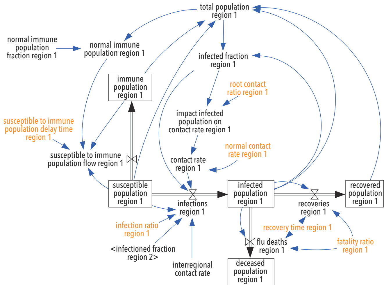
Figure 2. Exploratory system dynamics model of the flu in two regions (Pruyt and Hamarat 2010)
